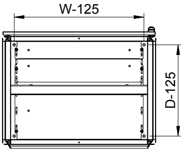
Sectional top view (without bottom plates)
