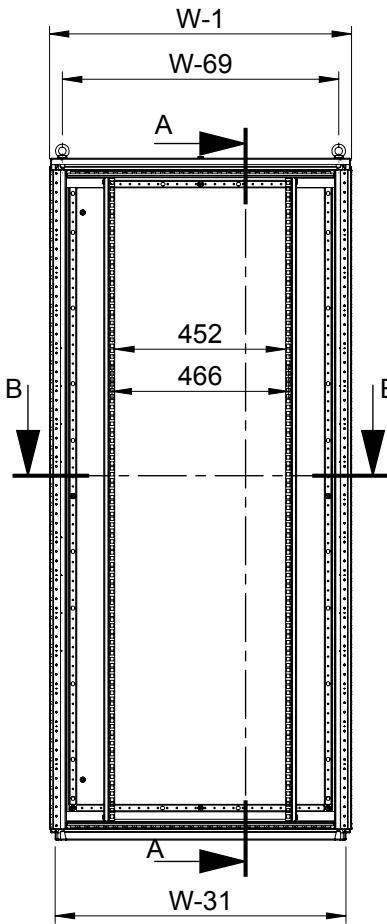
Front view
